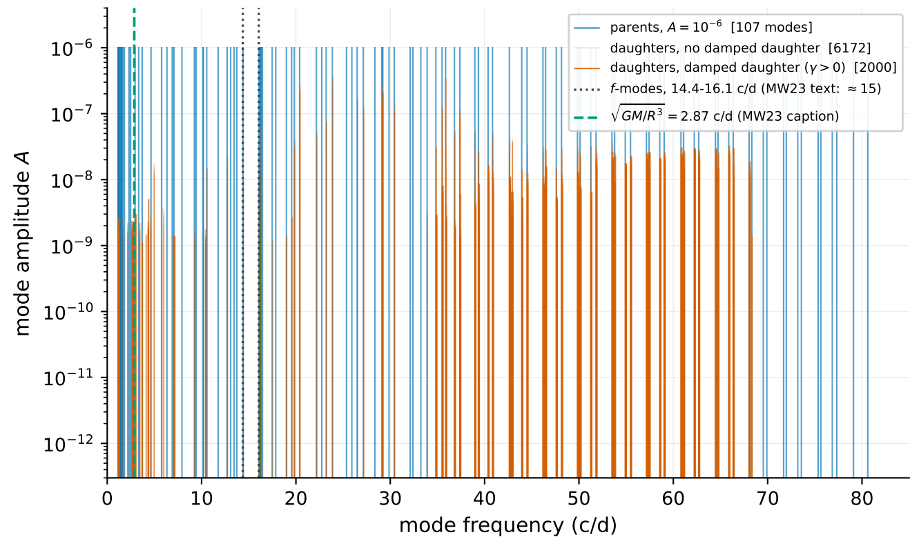
MW23 Fig. 6: 8172 triplets with \mu > 10^3 ; A_c = \mu A_a A_b at A_a = A_b = 10^{-6}
