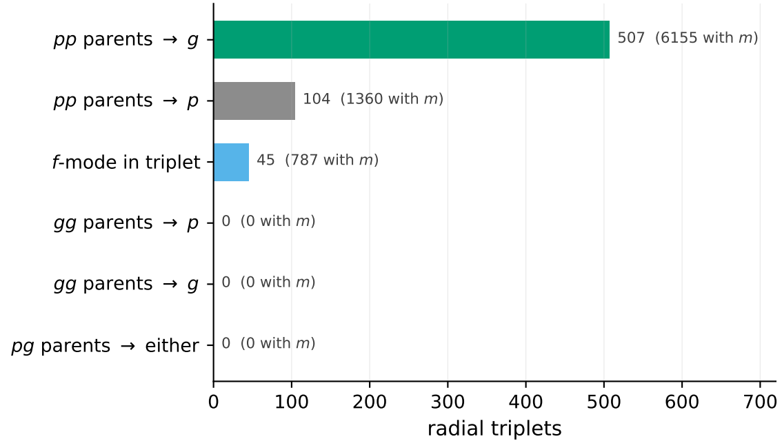
(b) direct: two parents \rightarrow one daughter 656 radial triplets
