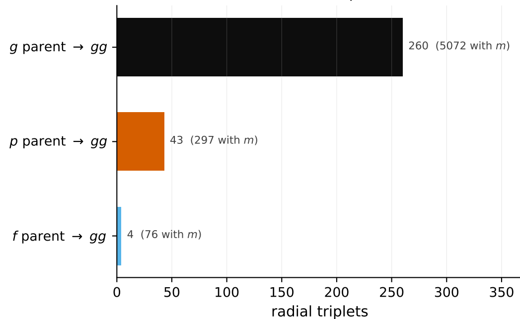
(a) parametric: one parent \rightarrow two daughters 307 radial triplets
