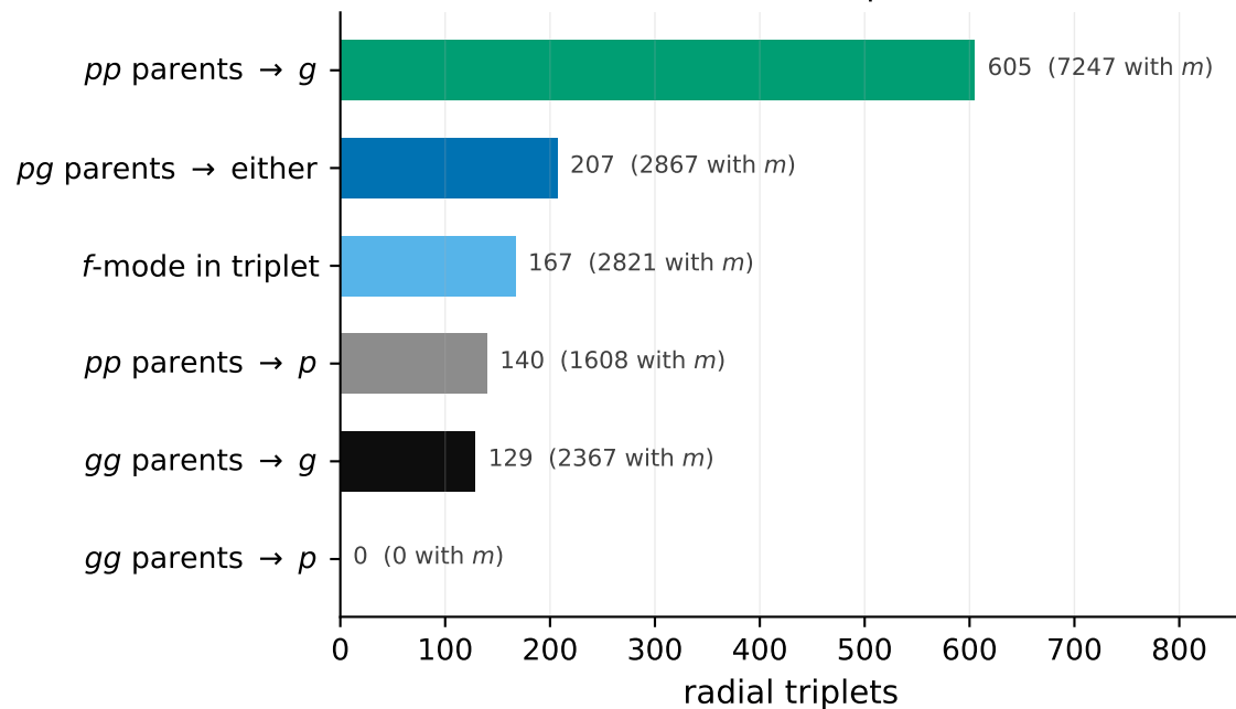
(b) direct: two parents \rightarrow one daughter 1248 radial triplets
