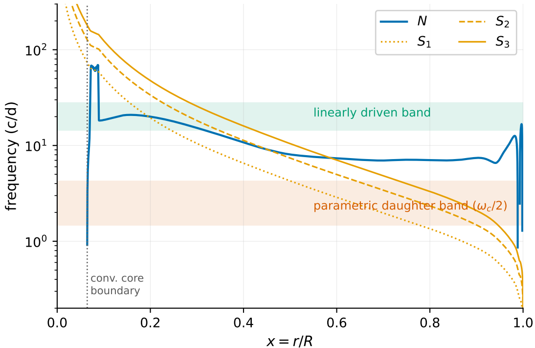
Propagation diagram, M = 2.20 M_{\odot} \delta Sct model
