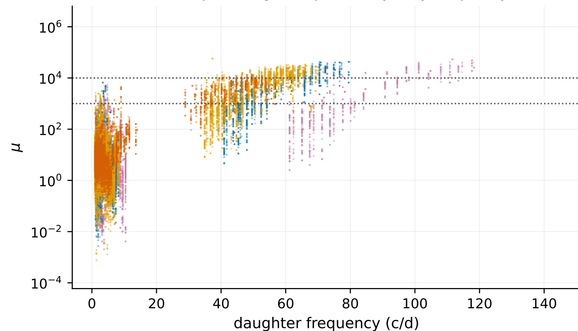
(b) damped daughter ( \gamma > 0 ) only -- by frequency
