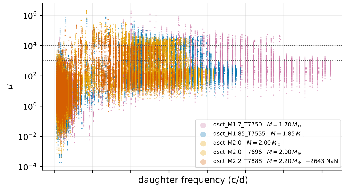
(b) damped daughter ( \gamma > 0 ) only -- by frequency
