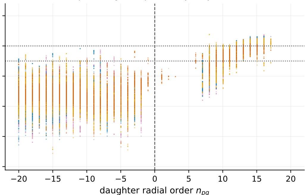
(b) damped daughter ( \gamma > 0 ) only -- by radial order
