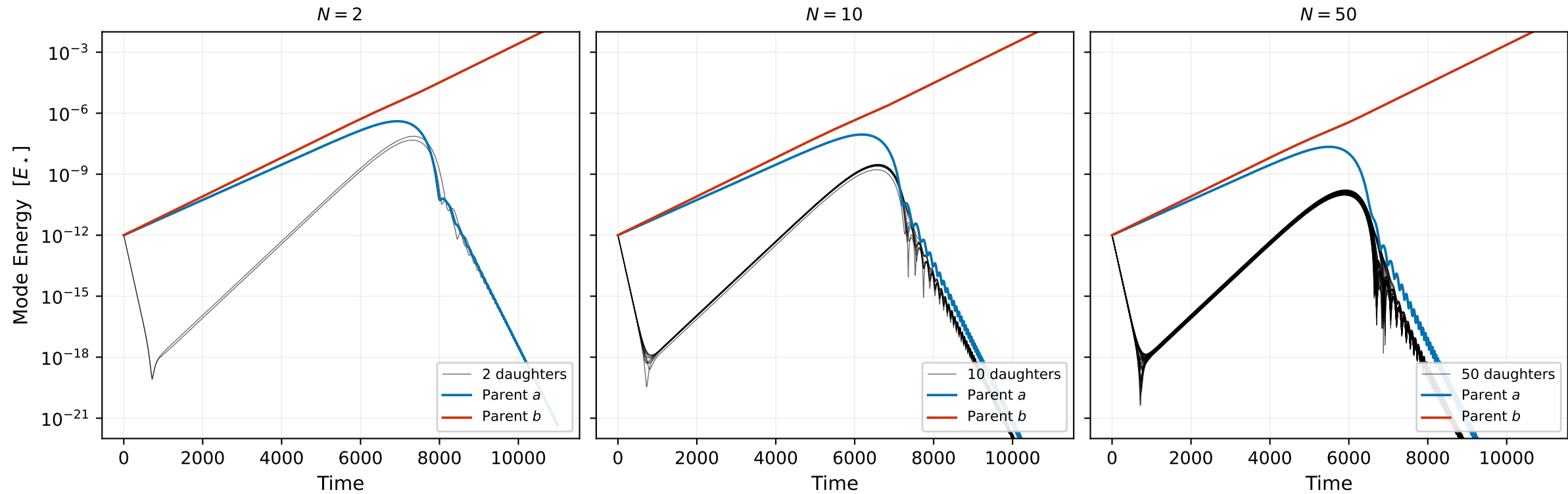
MW25 Figure 2 -- two parents, N damped daughters, still unstable [C++]
