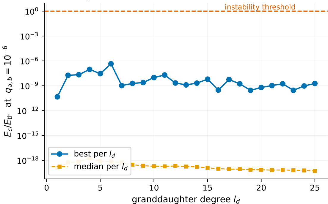
Four-mode systems, full net (2.2M candidates): all far below threshold
