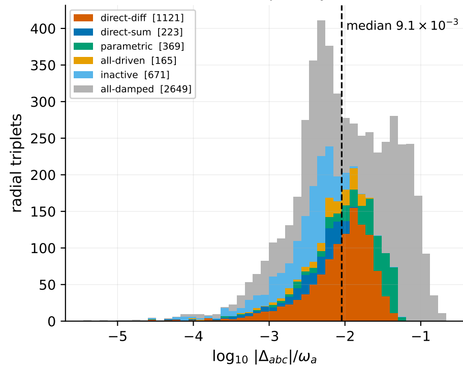
(a) 5198 radial triplets by channel
