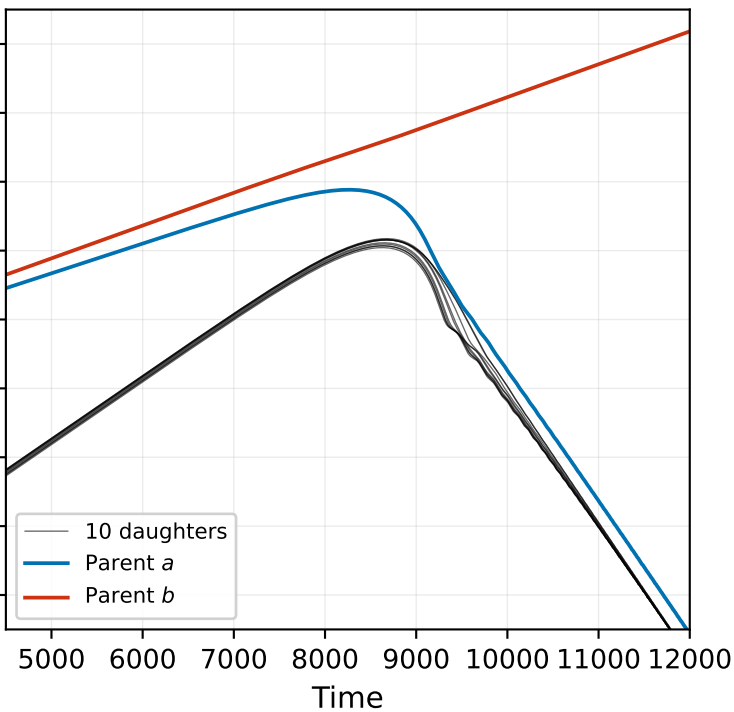
MW25 Figure 2 -- two parents, N damped daughters, still unstable
