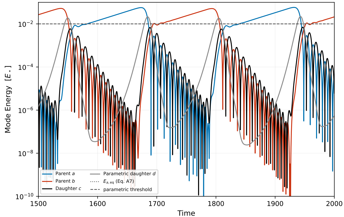
MW25 Figure 3 -- mixed direct + parametric coupling: limit cycle
