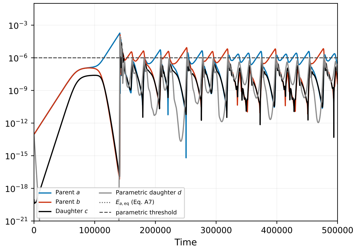
MW25 Figure 4 -- limit-cycle behaviour vs the parameters
