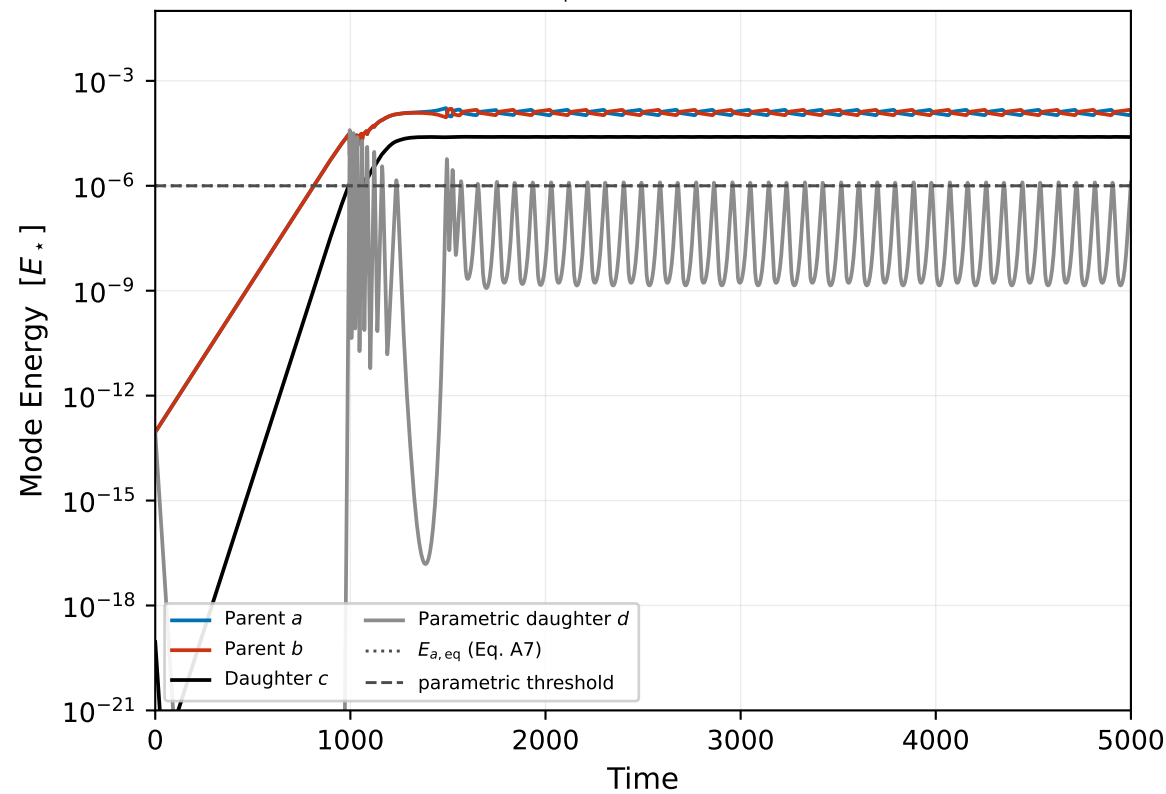
MW25 Figure 4 -- limit-cycle behaviour vs the parameters
