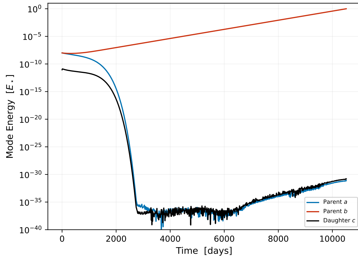
(a) direct triplet only: unstable
