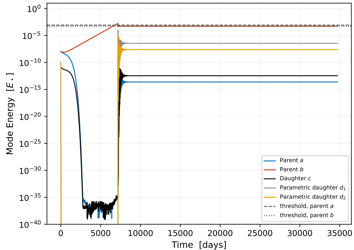
(b) five-mode mixed network
