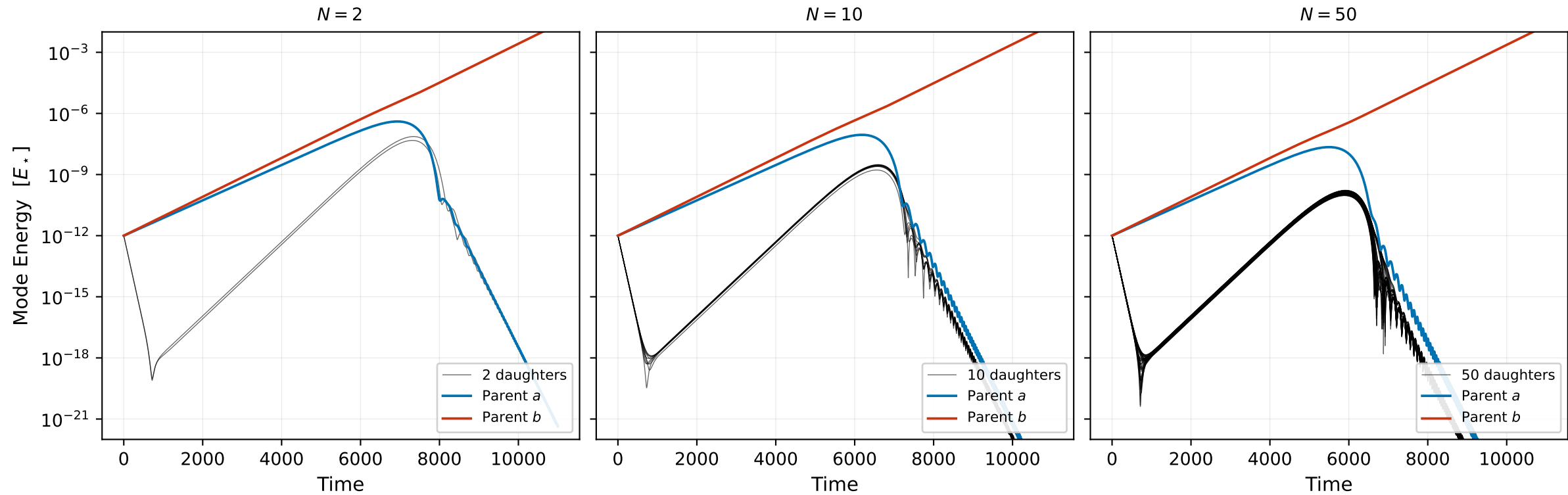
MW25 Figure 2 -- two parents, N damped daughters, still unstable
