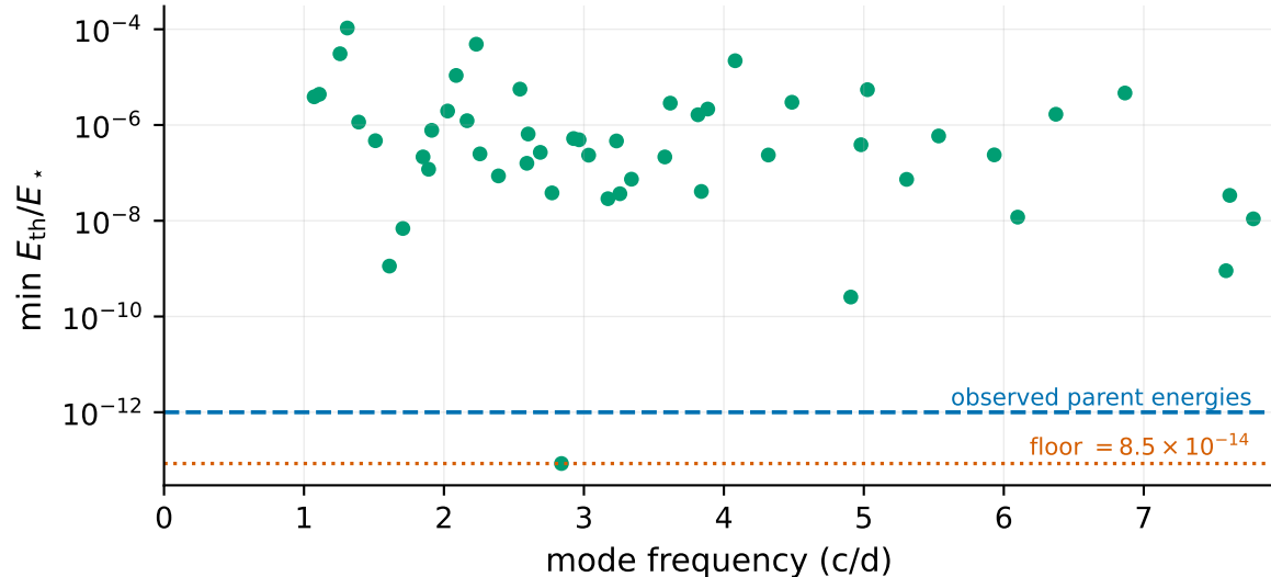
(b) parametric: 1 mode(s) reachable at observed parent energies
