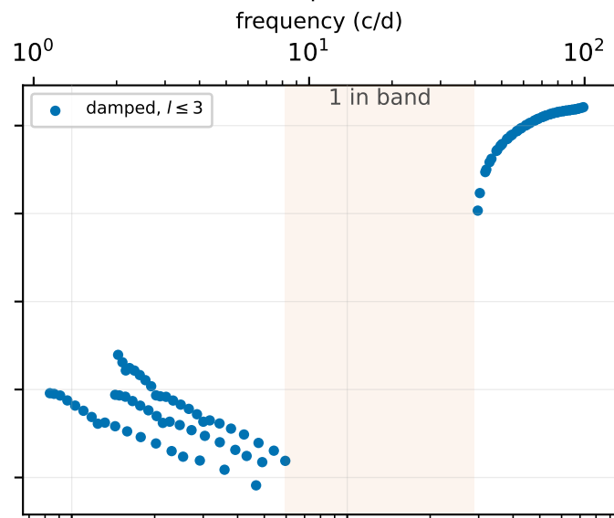
(b) damped, l \leq 3
