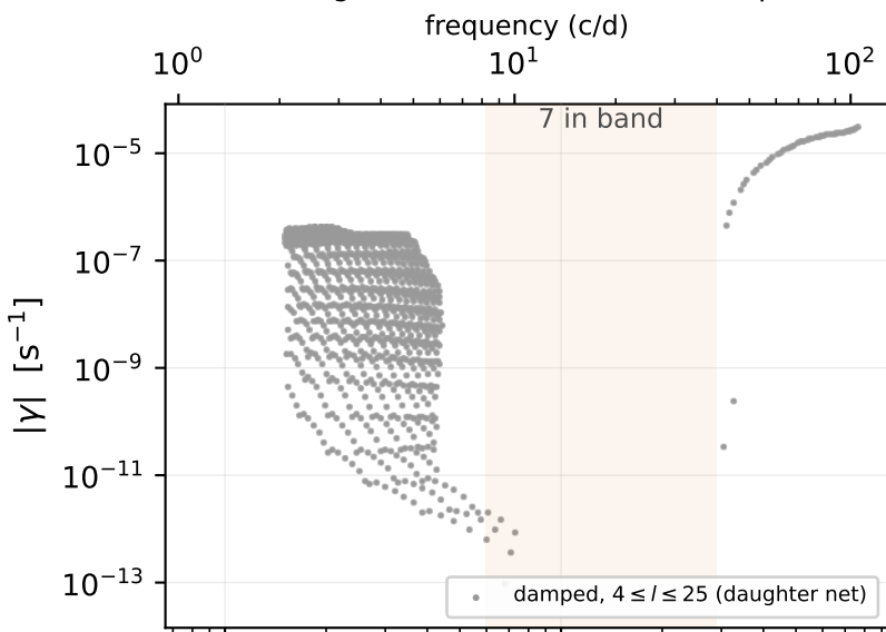
(a) daughter net, 4 \leq l \leq 25 (all damped)
