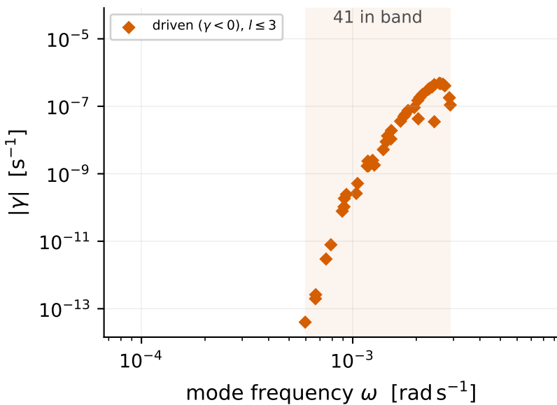
(c) driven, l \leq 3
