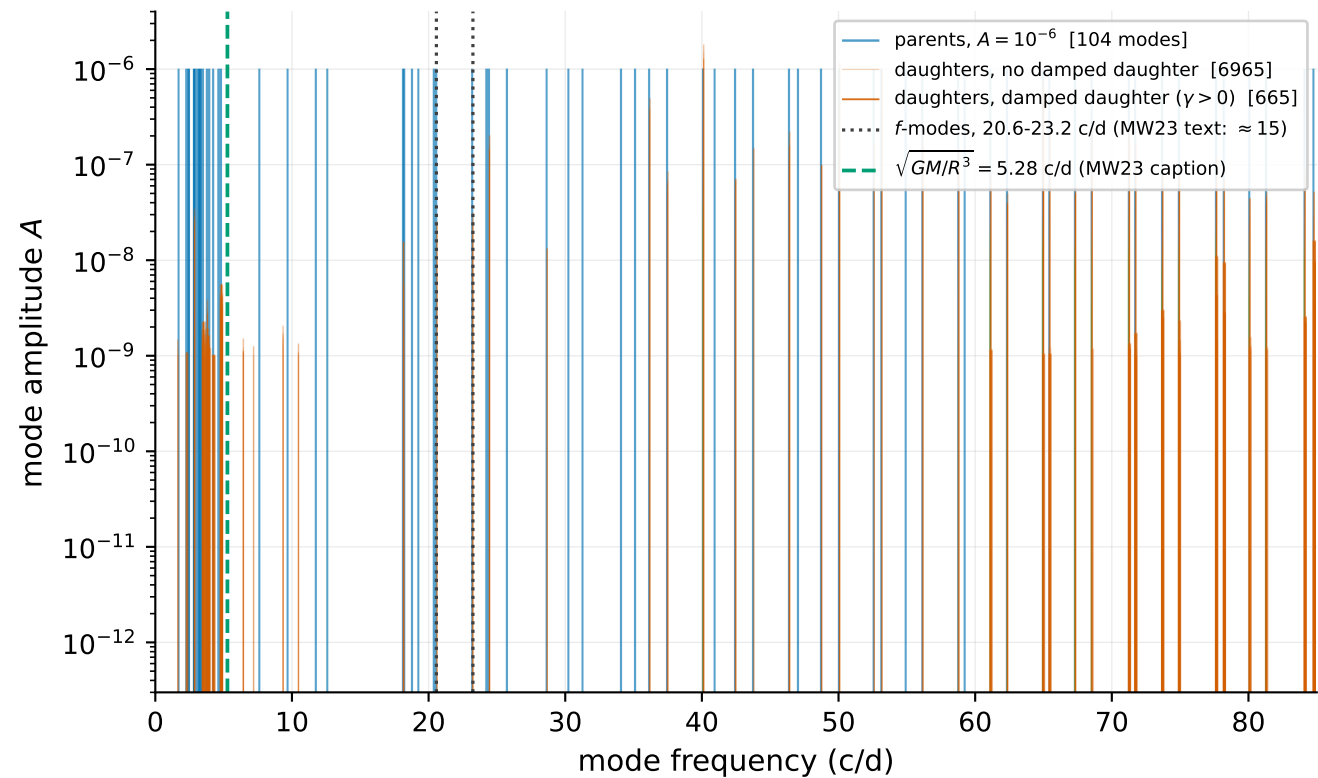
MW23 Fig. 6: 7630 triplets with \mu > 10^3 ; A_c = \mu A_a A_b at A_a = A_b = 10^{-6}
