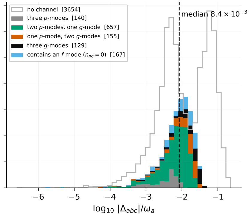
(b) 1248 direct radial triplets by p/g make-up
