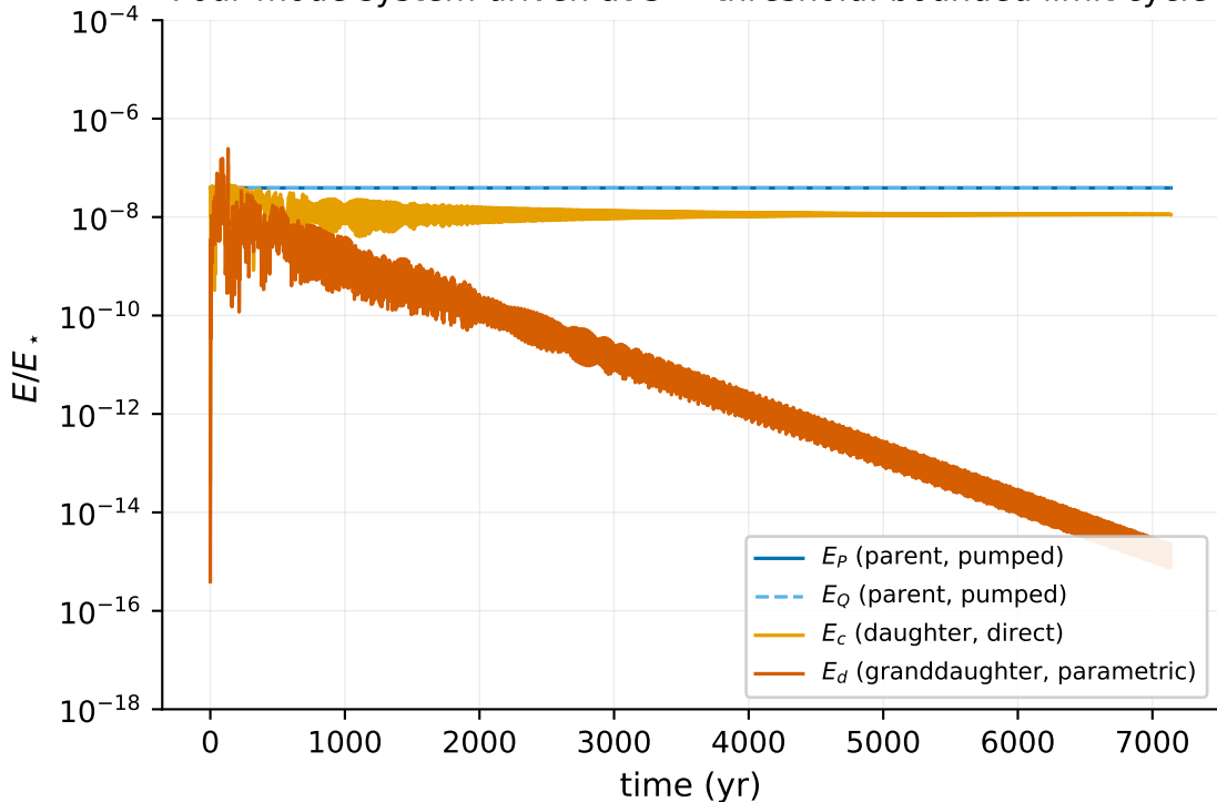
Four-mode system driven at 3 \times threshold: bounded limit cycle
