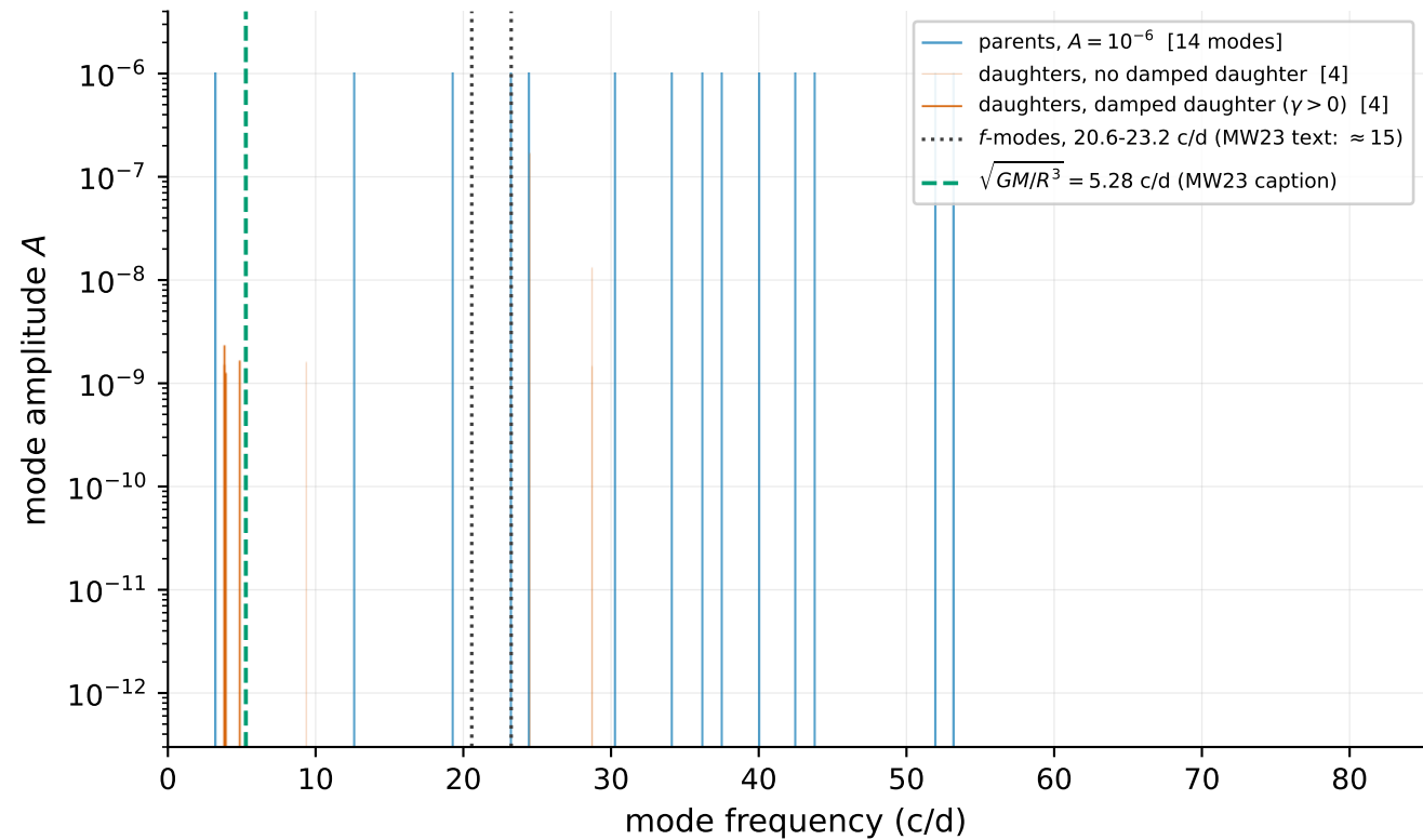
MW23 Fig. 6: 8 triplets with \mu > 10^3 ; A_c = \mu A_a A_b at A_a = A_b = 10^{-6}
