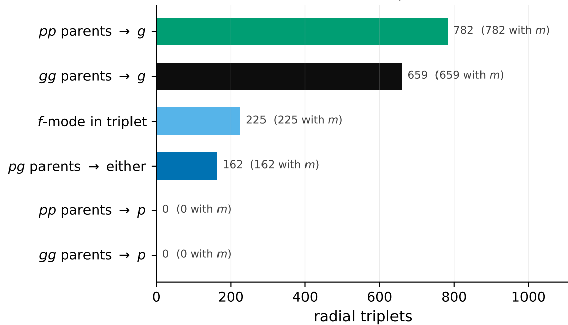
(b) direct: two parents \rightarrow one daughter 1828 radial triplets
