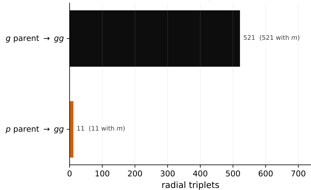
(a) parametric: one parent \rightarrow two daughters 532 radial triplets
