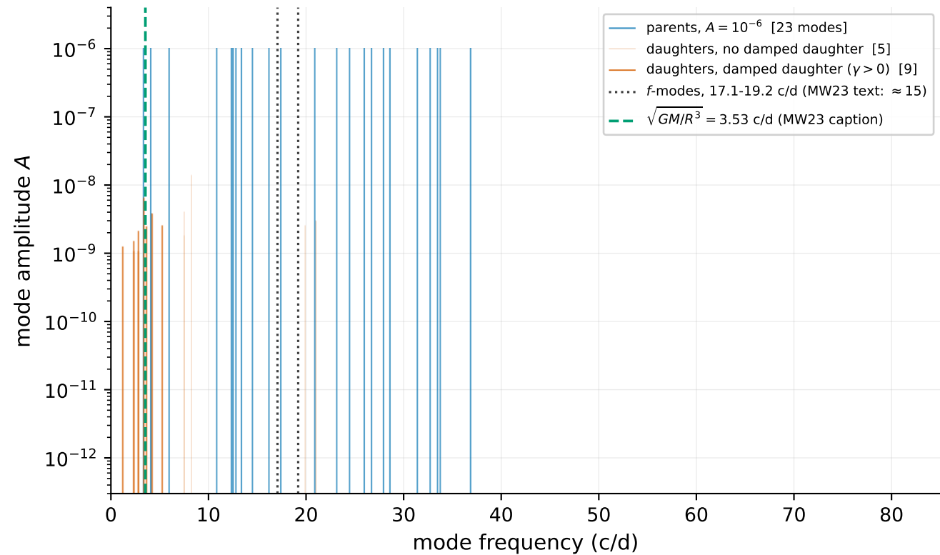
MW23 Fig. 6: 14 triplets with \mu > 10^3 ; A_c = \mu A_a A_b at A_a = A_b = 10^{-6}
