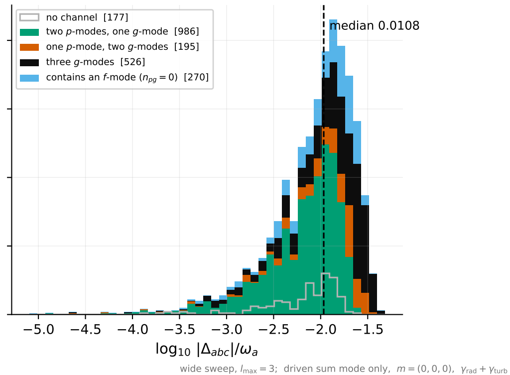
(b) 1977 direct radial triplets by p/g make-up
