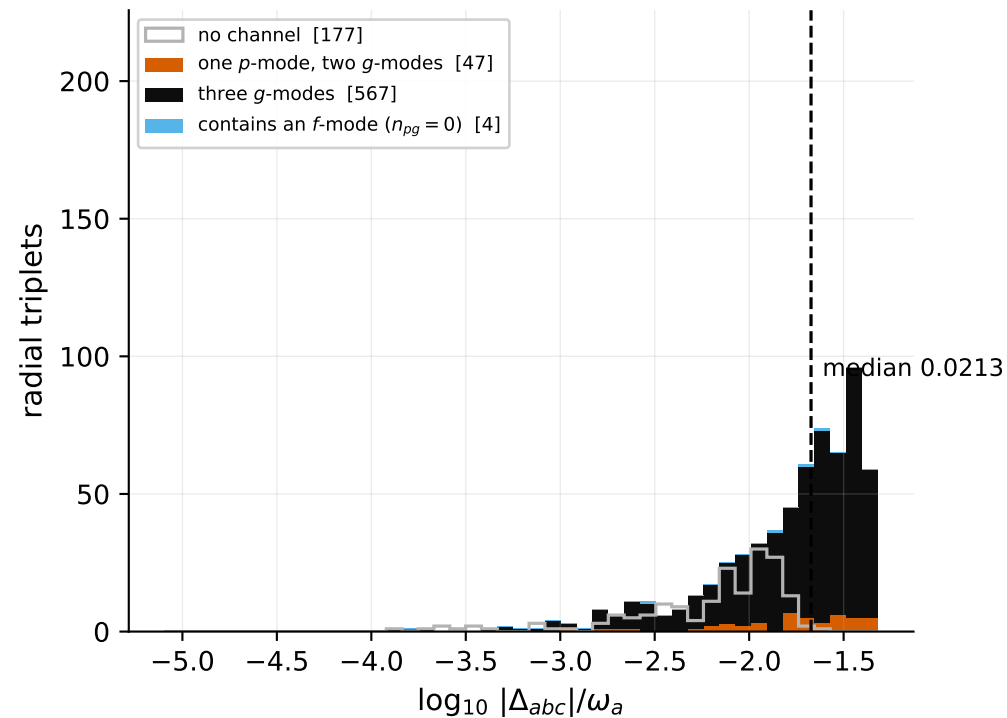
(a) 618 parametric radial triplets by p/g make-up
