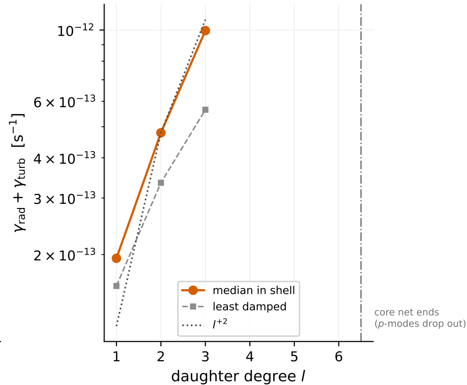
(b) daughter damping
