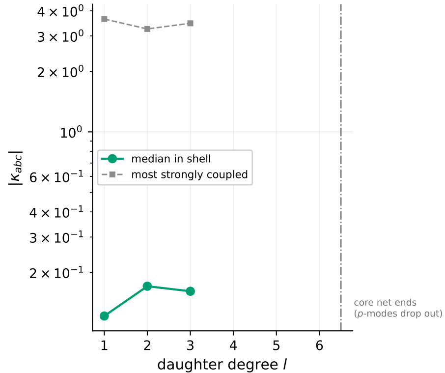
(c) coupling strength
