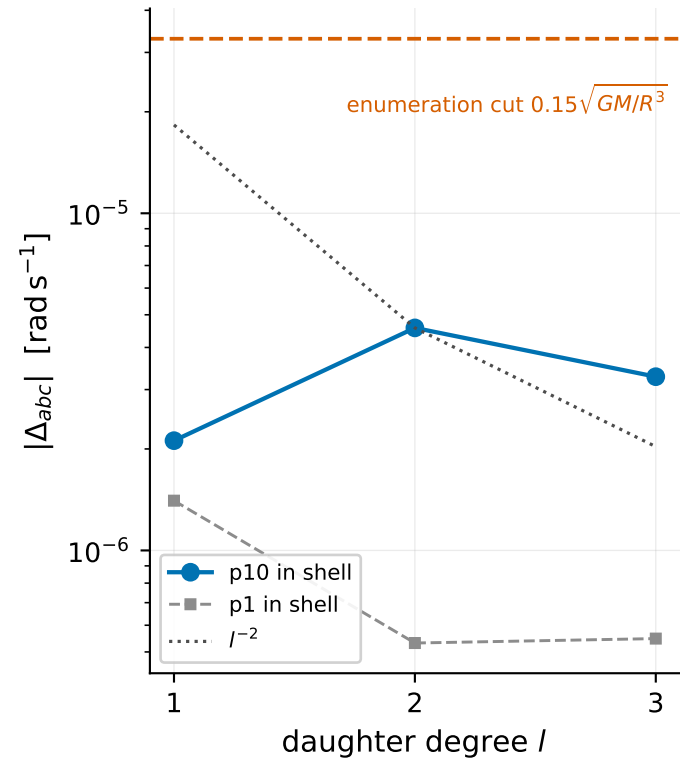
(a) achievable detuning
