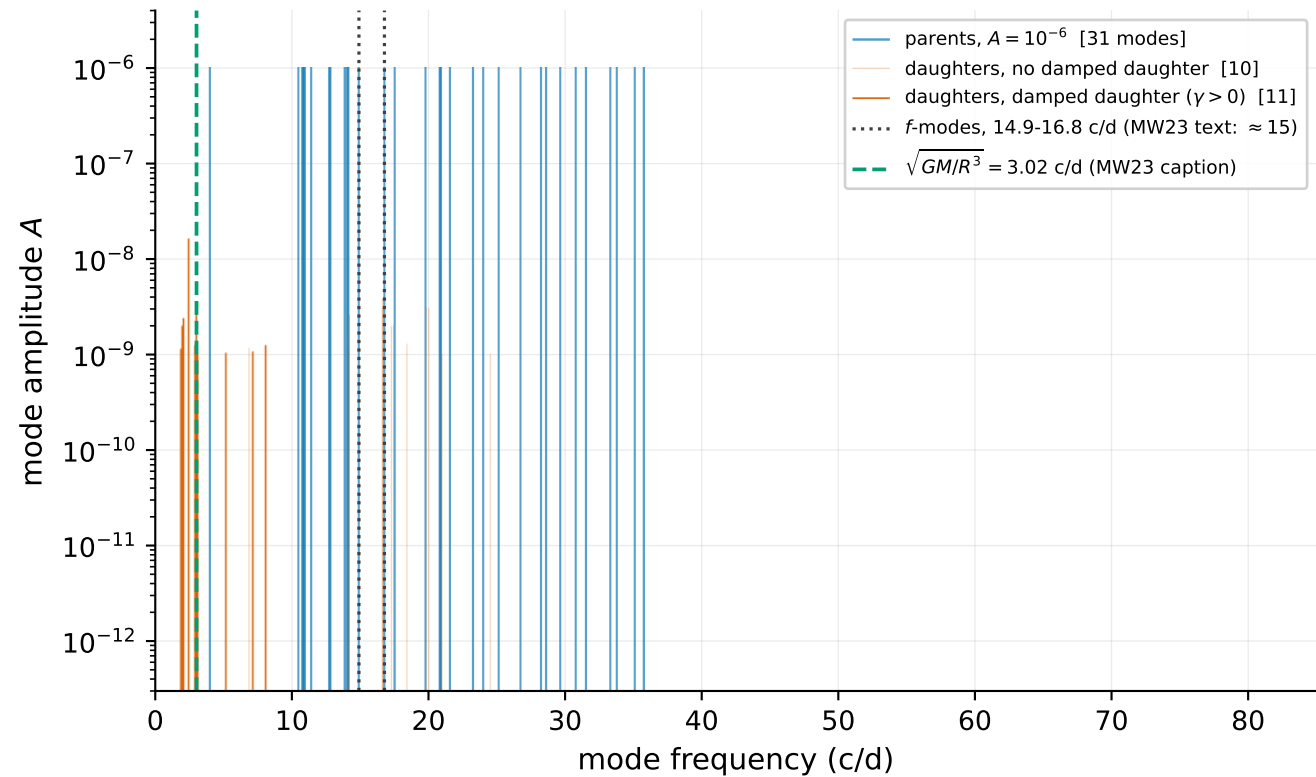
MW23 Fig. 6: 21 triplets with \mu > 10^3 ; A_c = \mu A_a A_b at A_a = A_b = 10^{-6}
