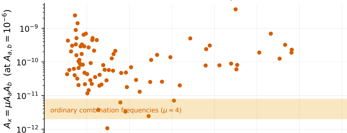
(b) parametric: every threshold sits 310x above observed
