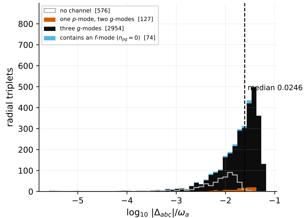
(a) 3155 parametric radial triplets by p/g make-up
