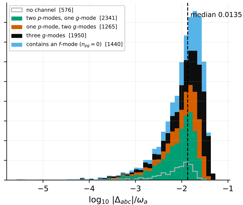
(b) 6996 direct radial triplets by p/g make-up
