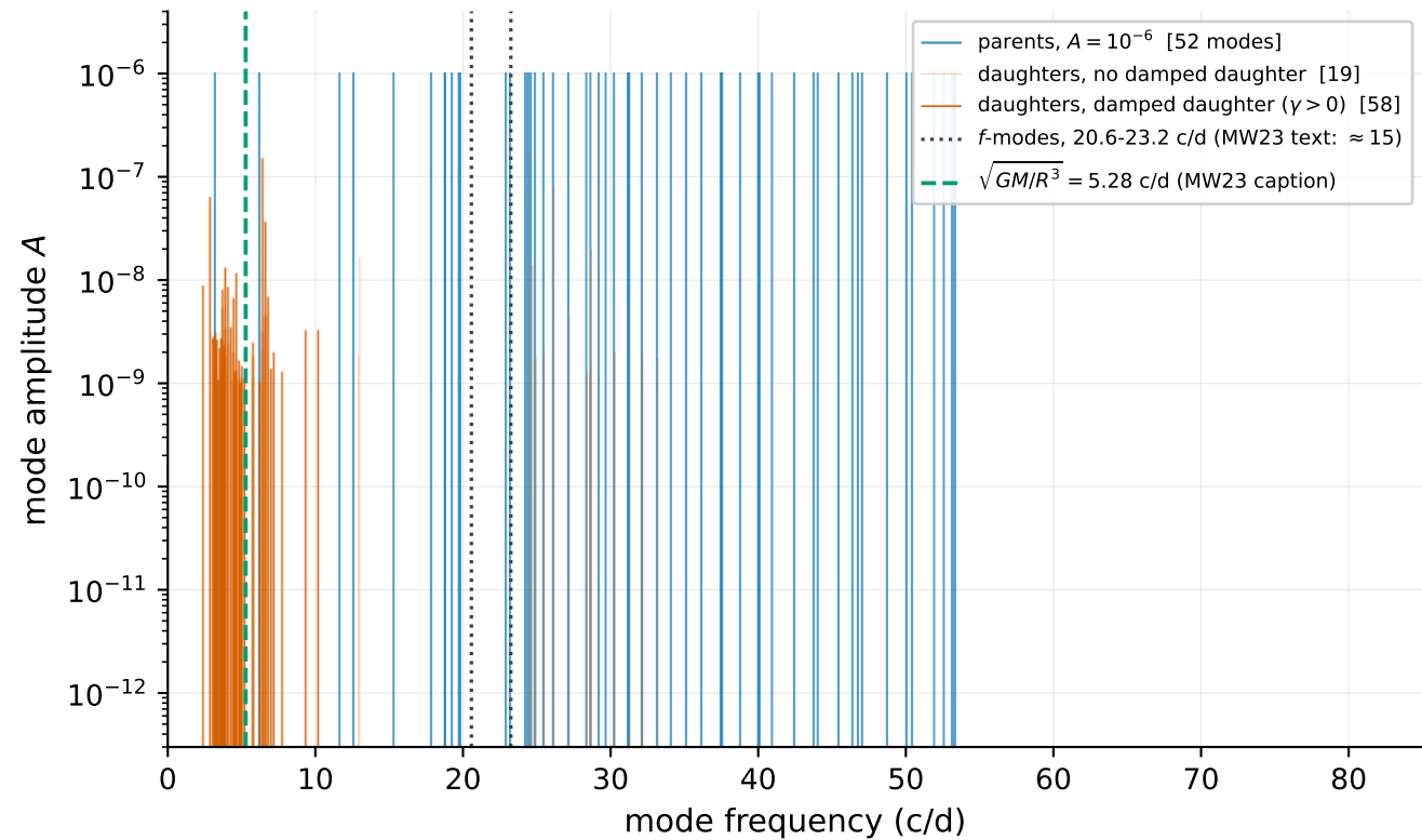
MW23 Fig. 6: 77 triplets with \mu > 10^3 ; A_c = \mu A_a A_b at A_a = A_b = 10^{-6}
