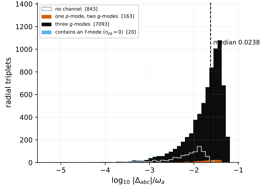
(a) 7276 parametric radial triplets by p/g make-up
