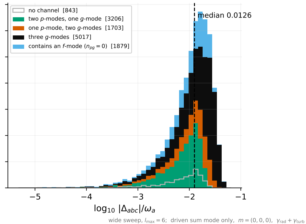
(b) 11805 direct radial triplets by p/g make-up
