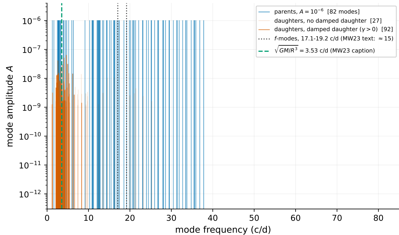
MW23 Fig. 6: 119 triplets with \mu > 10^3 ; A_c = \mu A_a A_b at A_a = A_b = 10^{-6}
