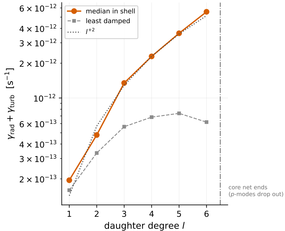
(b) daughter damping
