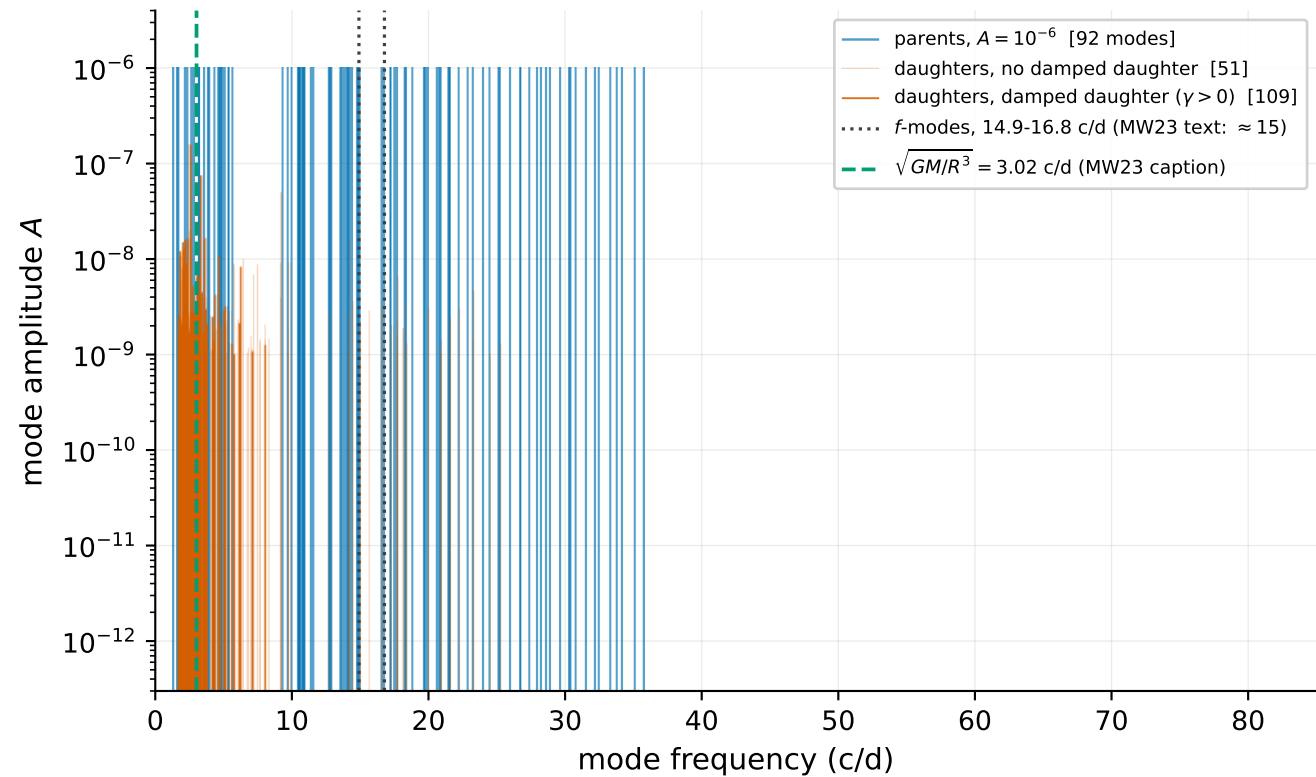
MW23 Fig. 6: 160 triplets with \mu > 10^3 ; A_c = \mu A_a A_b at A_a = A_b = 10^{-6}
