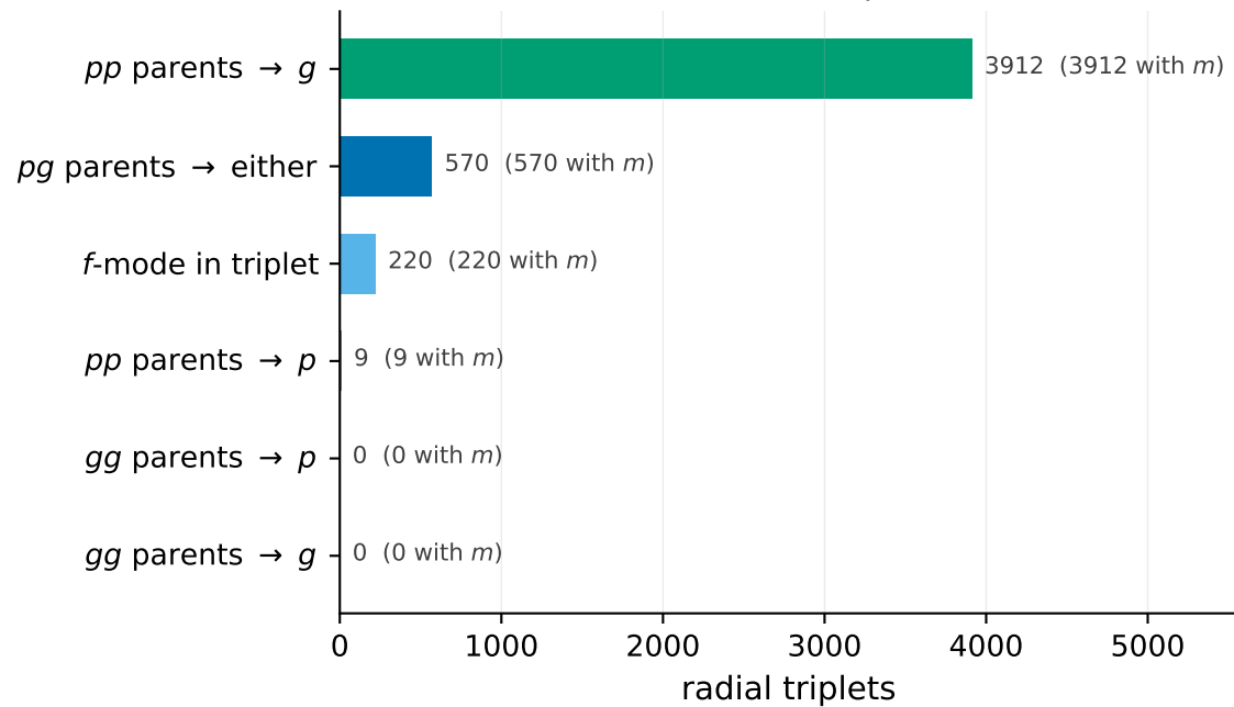
(b) direct: two parents \rightarrow one daughter 4711 radial triplets
