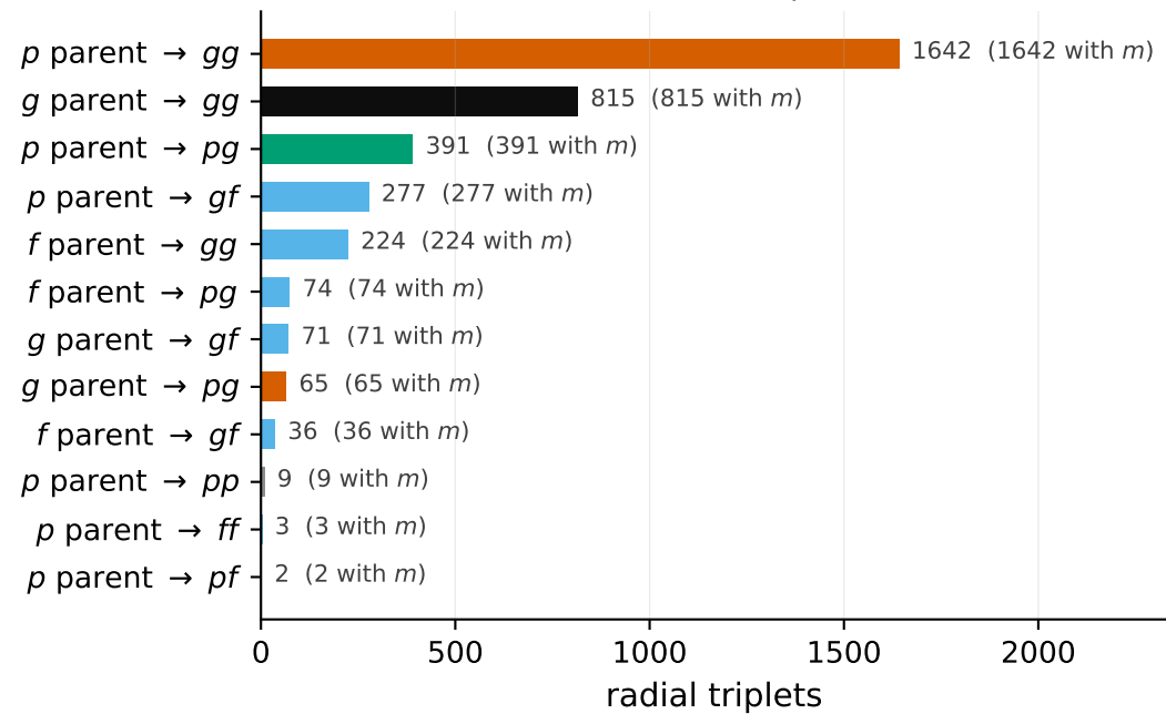
(a) parametric: one parent \rightarrow two daughters 3609 radial triplets
