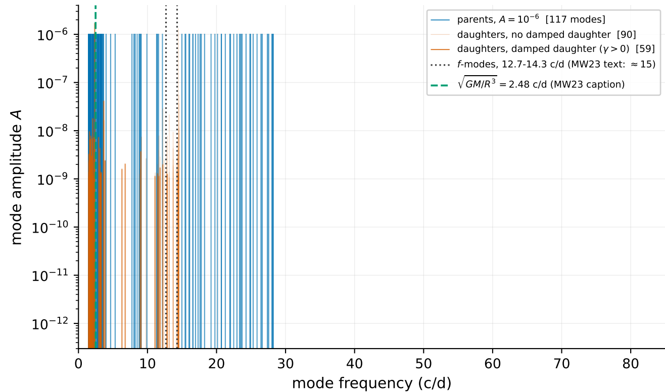
MW23 Fig. 6: 149 triplets with \mu > 10^3 ; A_c = \mu A_a A_b at A_a = A_b = 10^{-6}
