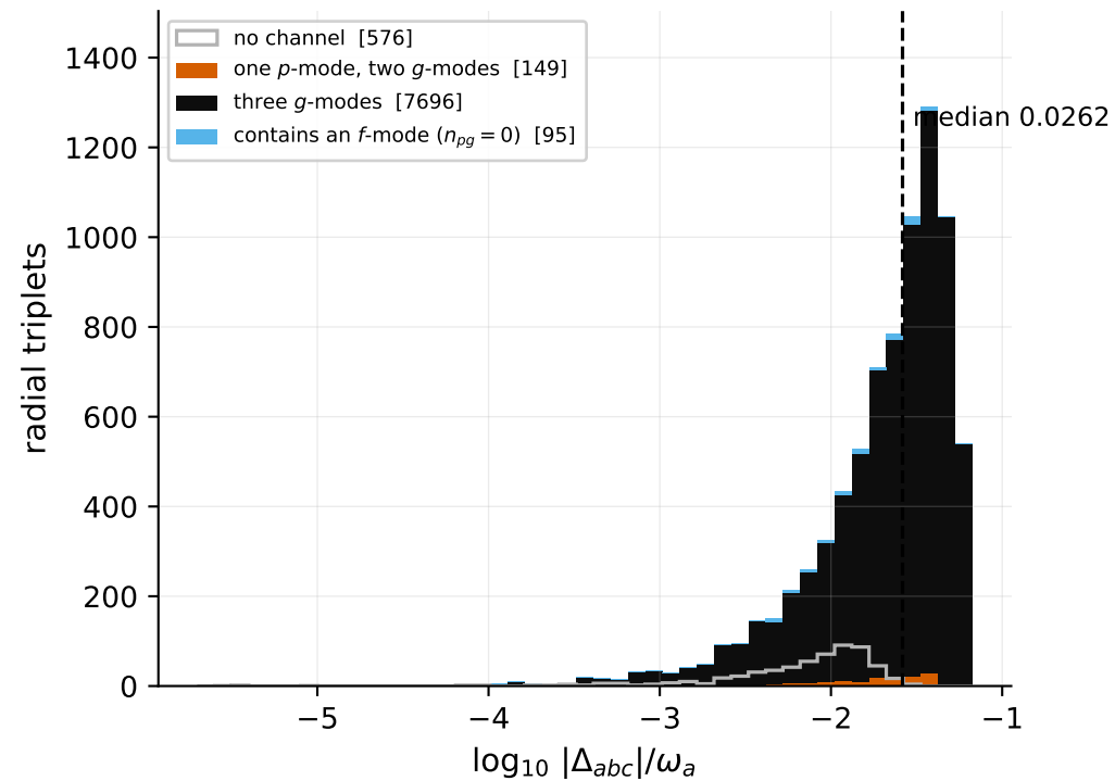
(a) 7940 parametric radial triplets by p/g make-up
