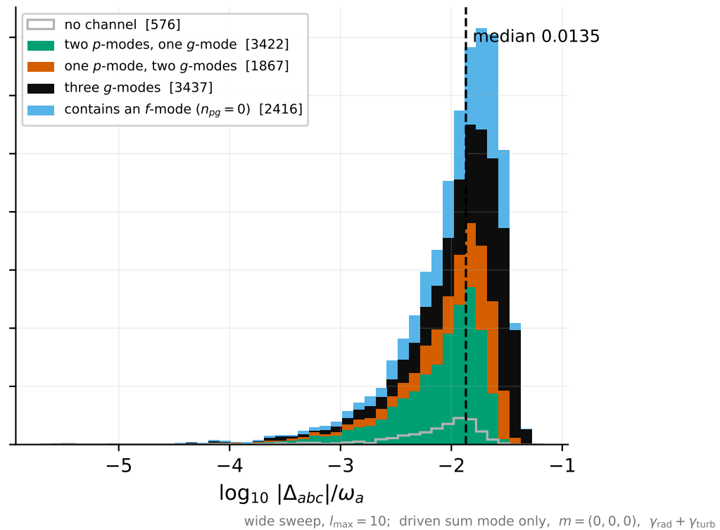
(b) 11142 direct radial triplets by p/g make-up
