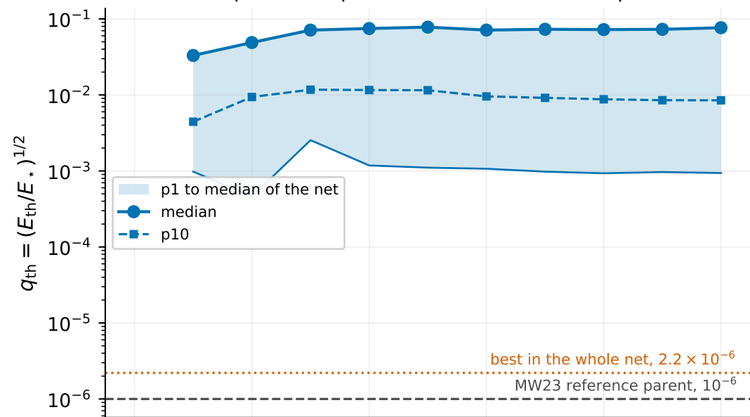
(c) triplets that can reach an equilibrium at all
