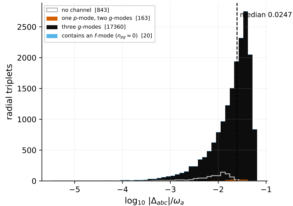
(a) 17543 parametric radial triplets by p/g make-up
