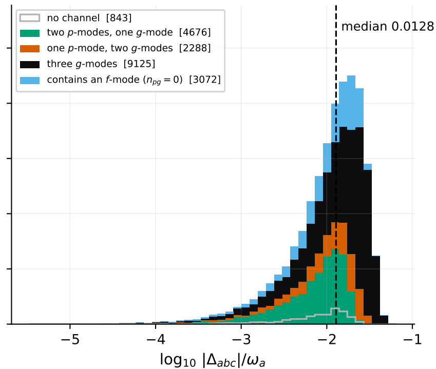
(b) 19161 direct radial triplets by p/g make-up
