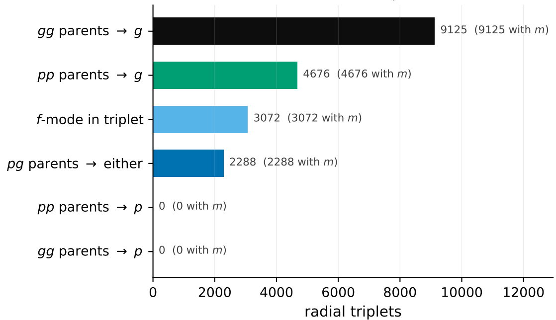
(b) direct: two parents \rightarrow one daughter 19161 radial triplets
