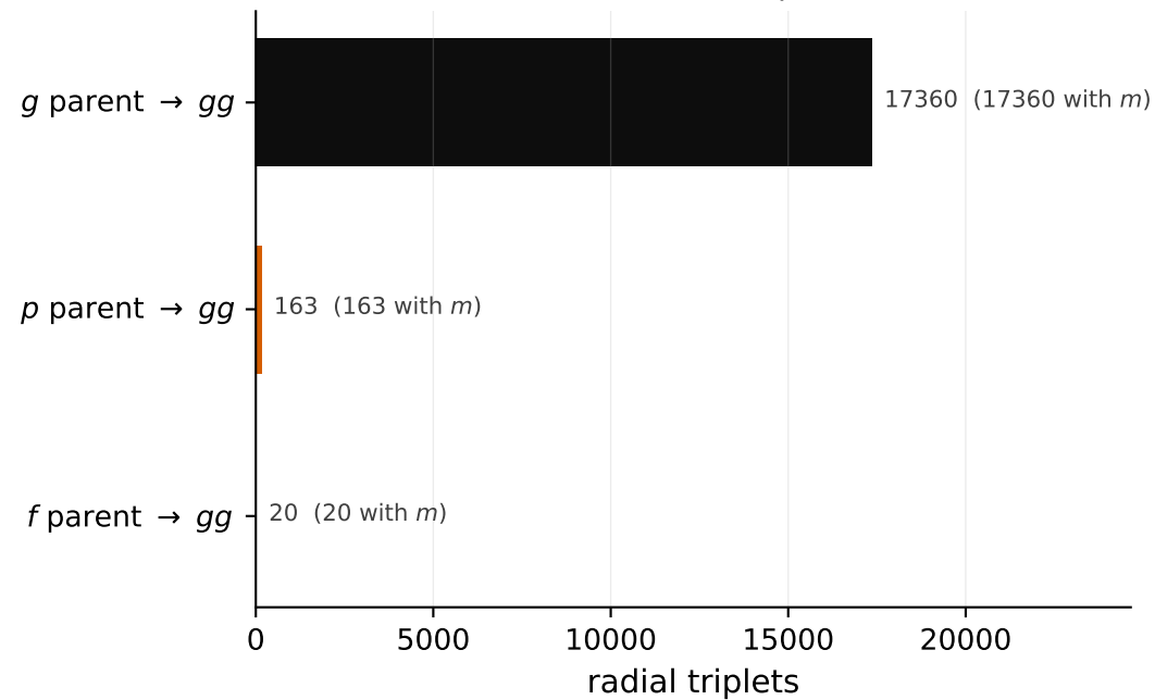
(a) parametric: one parent \rightarrow two daughters 17543 radial triplets
