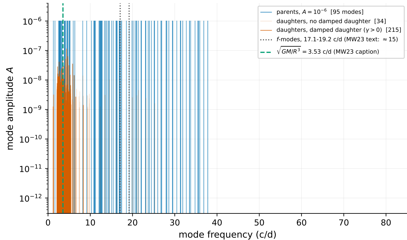
MW23 Fig. 6: 249 triplets with \mu > 10^3 ; A_c = \mu A_a A_b at A_a = A_b = 10^{-6}
