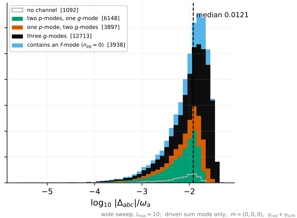
(b) 26696 direct radial triplets by p/g make-up
