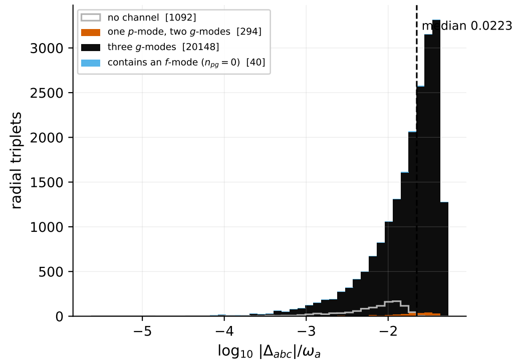
(a) 20482 parametric radial triplets by p/g make-up
