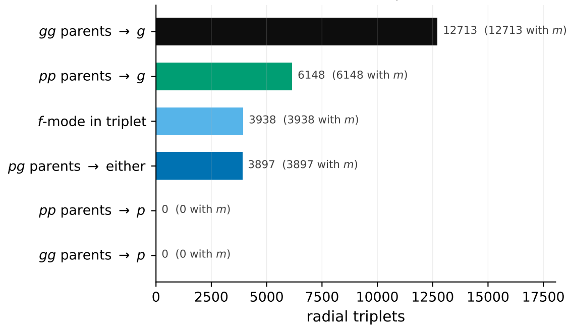
(b) direct: two parents \rightarrow one daughter 26696 radial triplets
