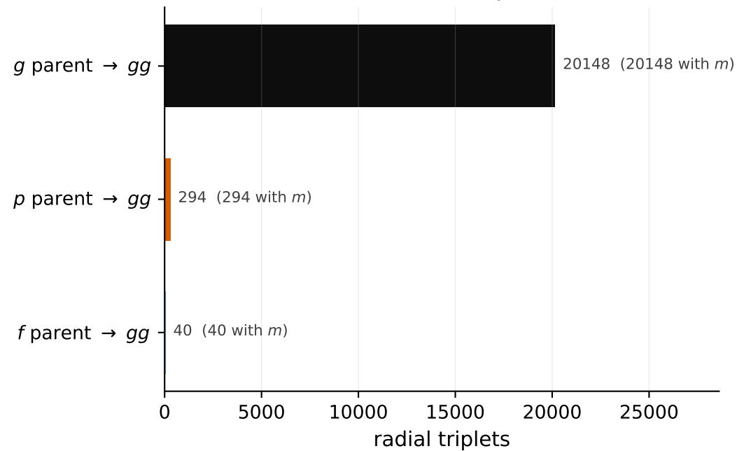
(a) parametric: one parent \rightarrow two daughters 20482 radial triplets
