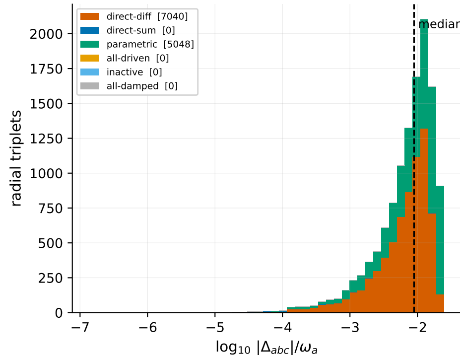
(a) 12088 radial triplets by channel
