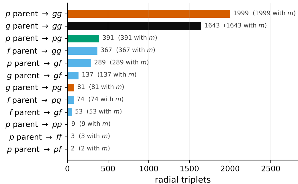
(a) parametric: one parent \rightarrow two daughters 5048 radial triplets
