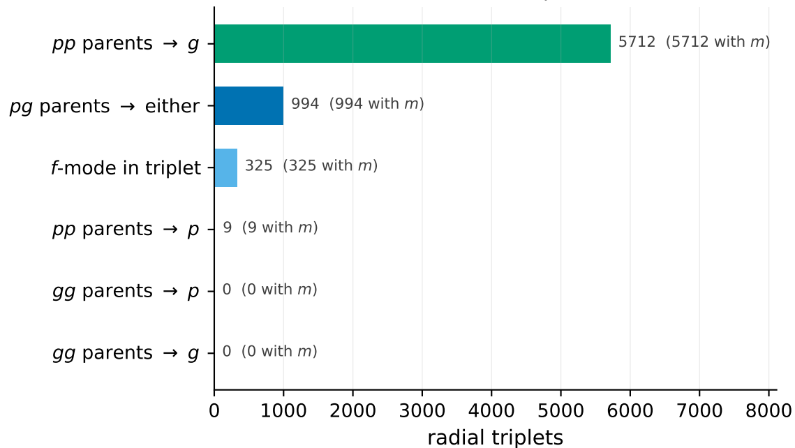
(b) direct: two parents \rightarrow one daughter 7040 radial triplets
