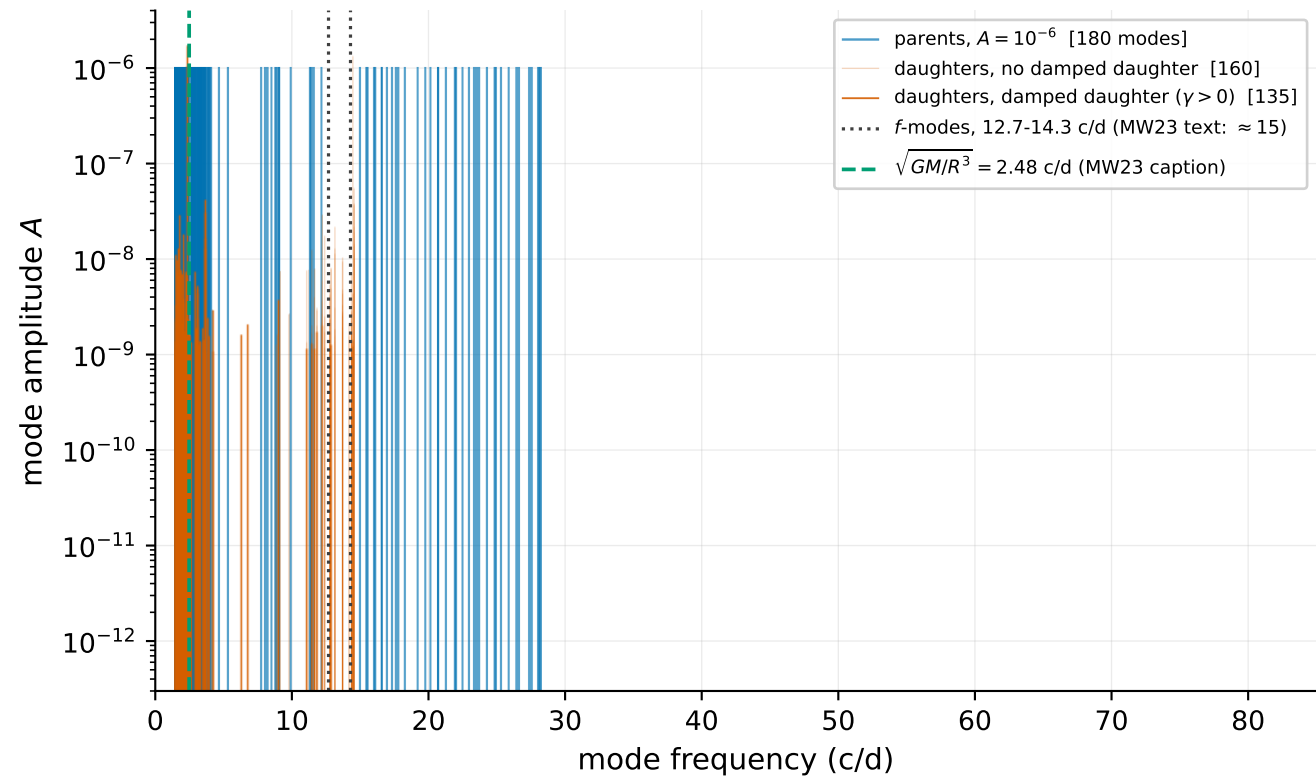
MW23 Fig. 6: 295 triplets with \mu > 10^3 ; A_c = \mu A_a A_b at A_a = A_b = 10^{-6}
