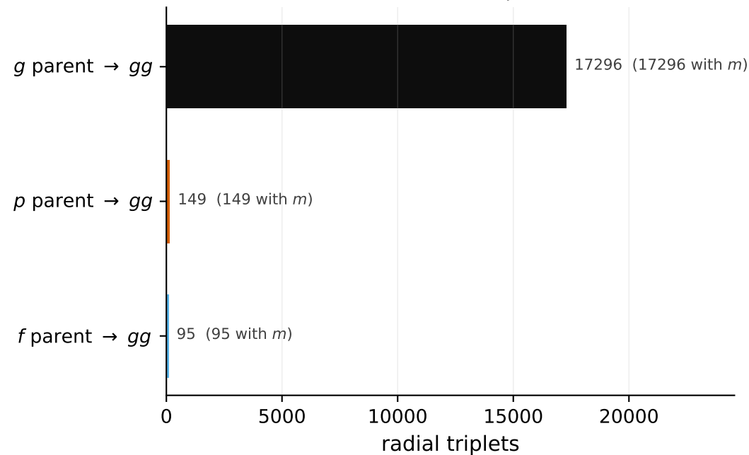
(a) parametric: one parent \rightarrow two daughters 17540 radial triplets
