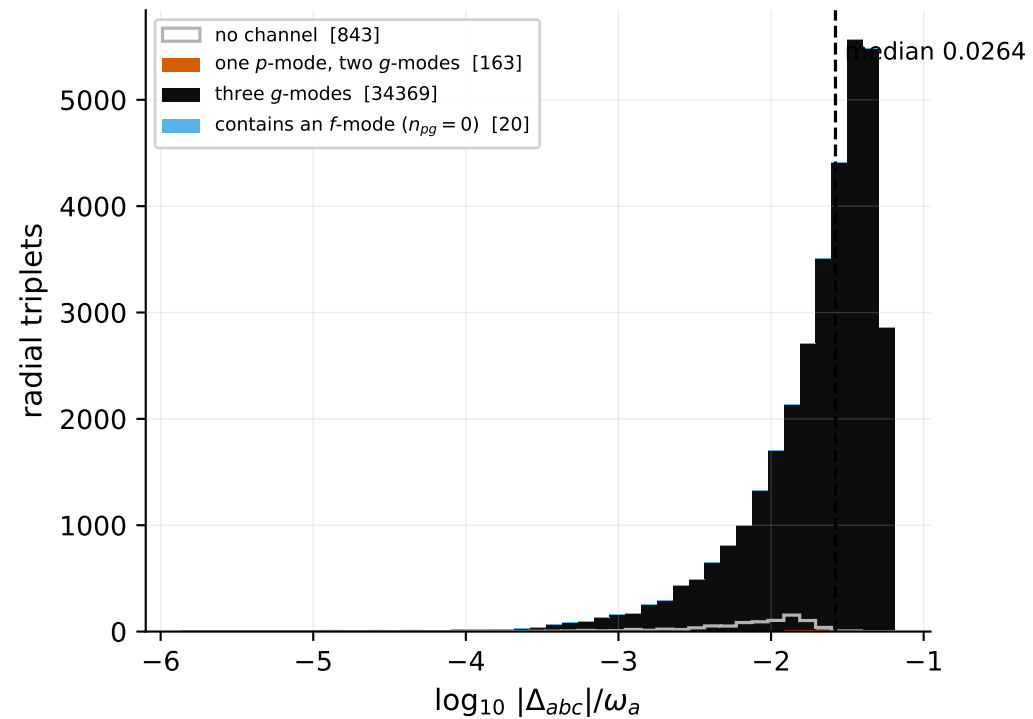
(a) 34552 parametric radial triplets by p/g make-up
