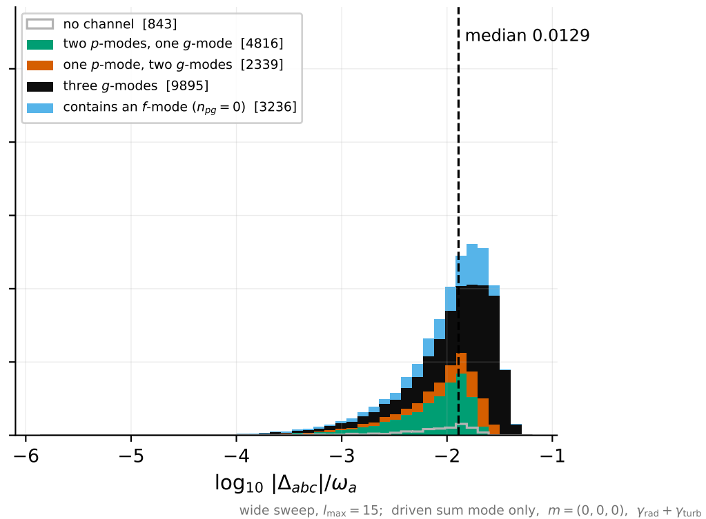
(b) 20286 direct radial triplets by p/g make-up
