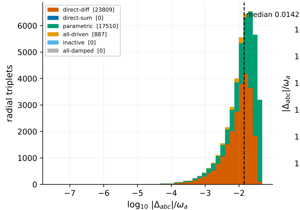
(a) 42206 radial triplets by channel
