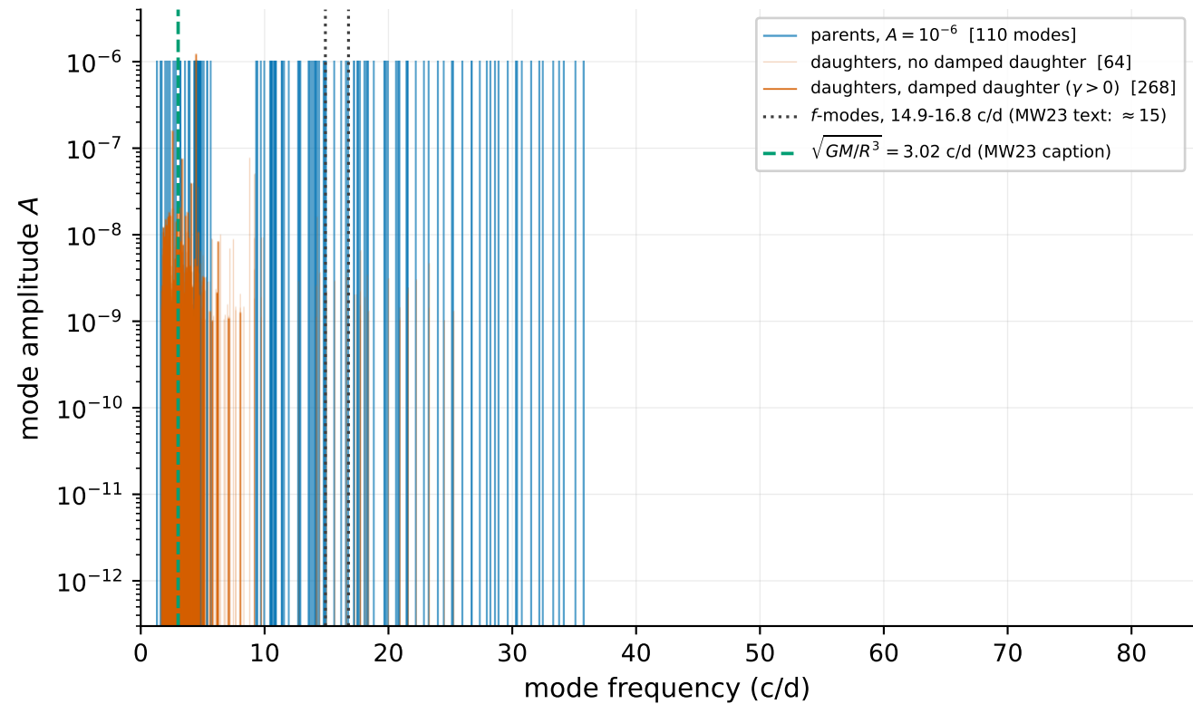
MW23 Fig. 6: 332 triplets with \mu > 10^3 ; A_c = \mu A_a A_b at A_a = A_b = 10^{-6}
