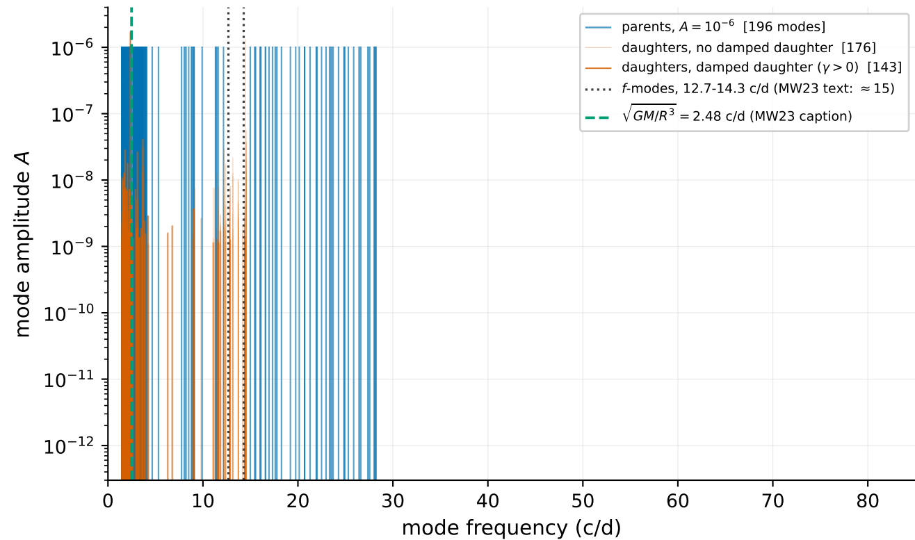
MW23 Fig. 6: 319 triplets with \mu > 10^3 ; A_c = \mu A_a A_b at A_a = A_b = 10^{-6}
