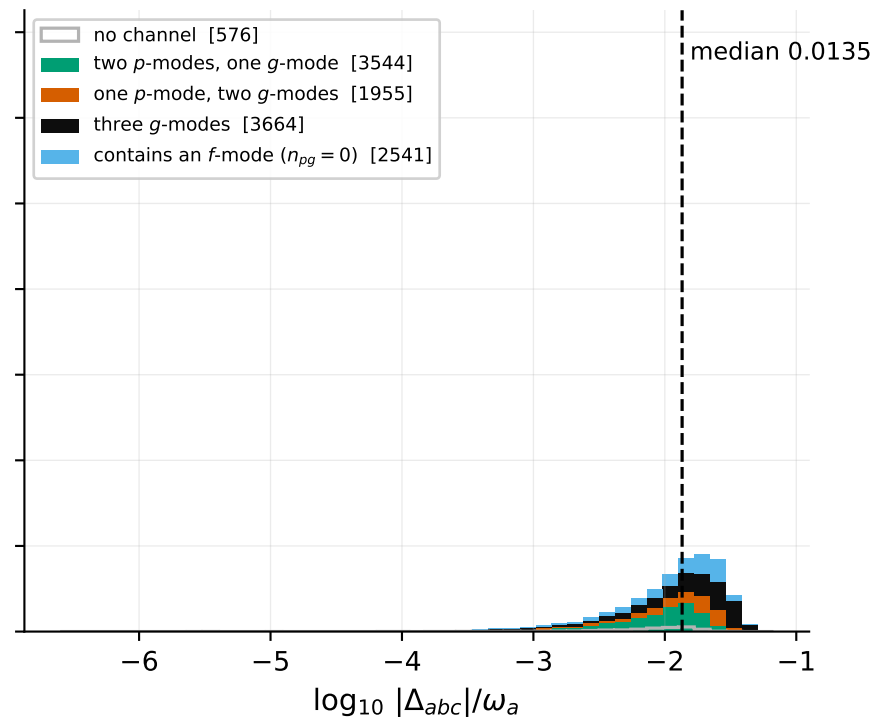
(b) 11704 direct radial triplets by p/g make-up
