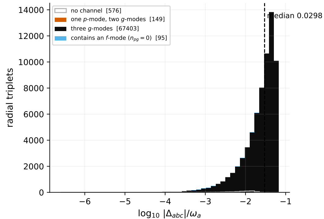
(a) 67647 parametric radial triplets by p/g make-up
