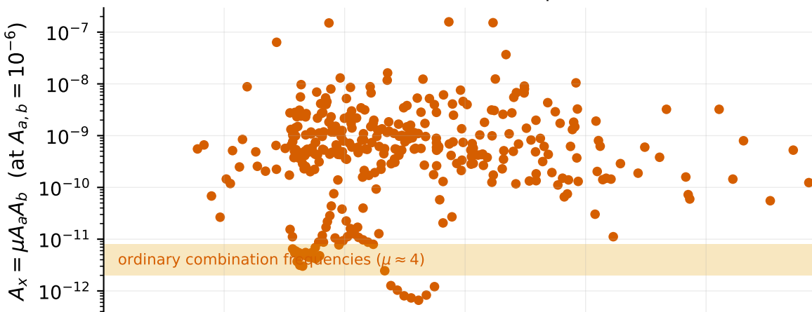
(b) parametric: every threshold sits 5x above observed
