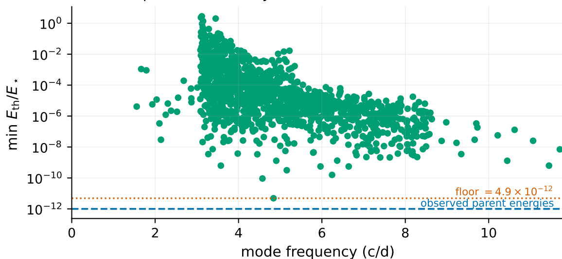
(b) parametric: every threshold sits 5x above observed
